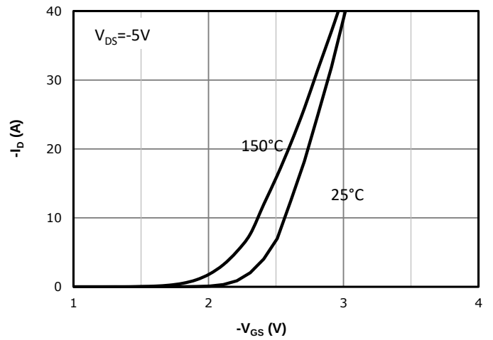
Fig 2: Transfer Characteristics
