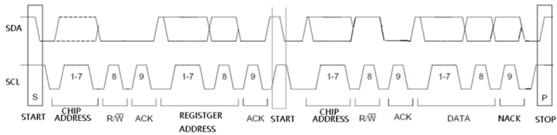
Figure 1b I 2 C Read Timing
