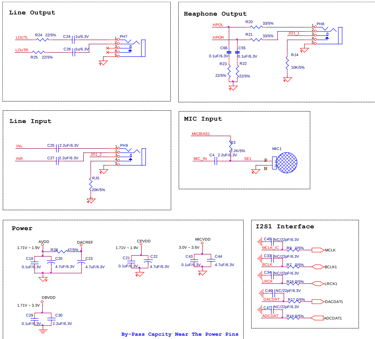
Figure 27. Application Circuit
