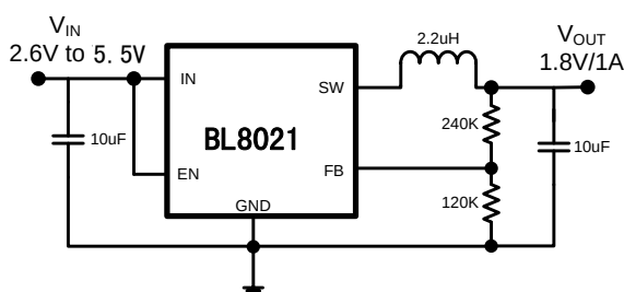
1.8V/1A Step-Down Converter
