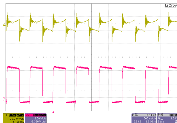
Output Ripple and SW at 1A load V_{in}=5V / V_{out}=2.5V
