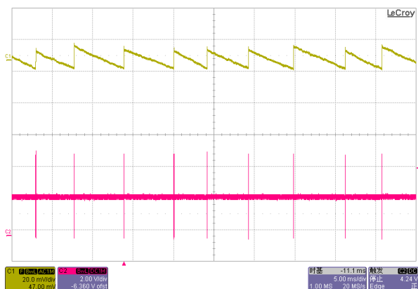
Output Ripple and SW at no load V_{in}=5V / V_{out}=2.5V
