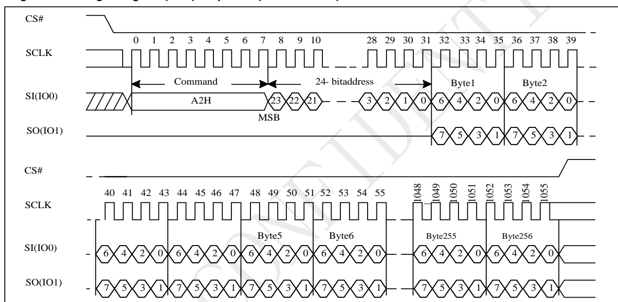
Figure 10-23 Page Program (DPP) Sequence (Command A2)
