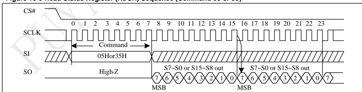
Status Register
