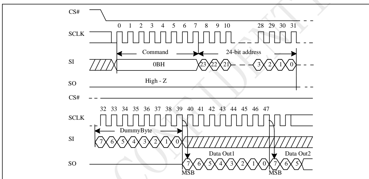
Figure 10-11 Read at Higher Speed (FAST_READ) Sequence (Command 0B)
