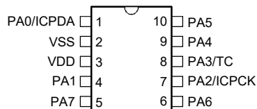
HT68F0017 10 SOP-A
