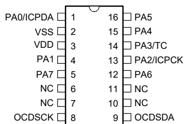
HT68V0017 16 NSOP-A
