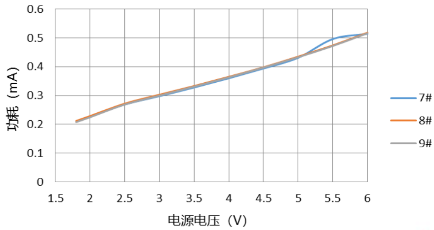
IDD功耗VS电源电压@FCPU=1MHz@HIRC
